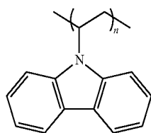
PVK (polyvinylcarbazole)
